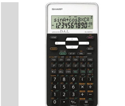
MATHEMATICS
